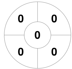
PINOKE
